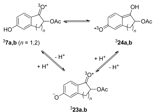
Scheme 8. Observed Transients in the LFP Experiments
